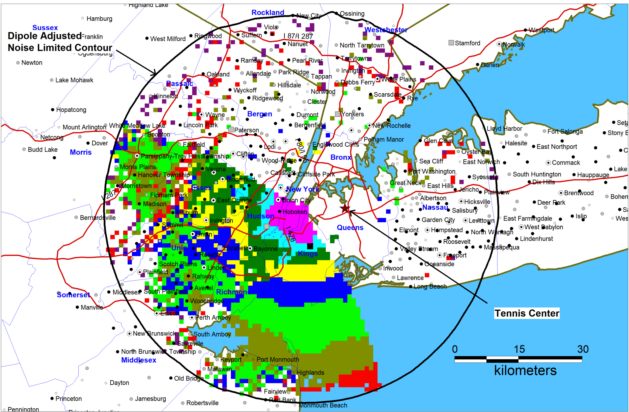
WKOB-LD New York, NC LIC Channel 2 Predicted Service
