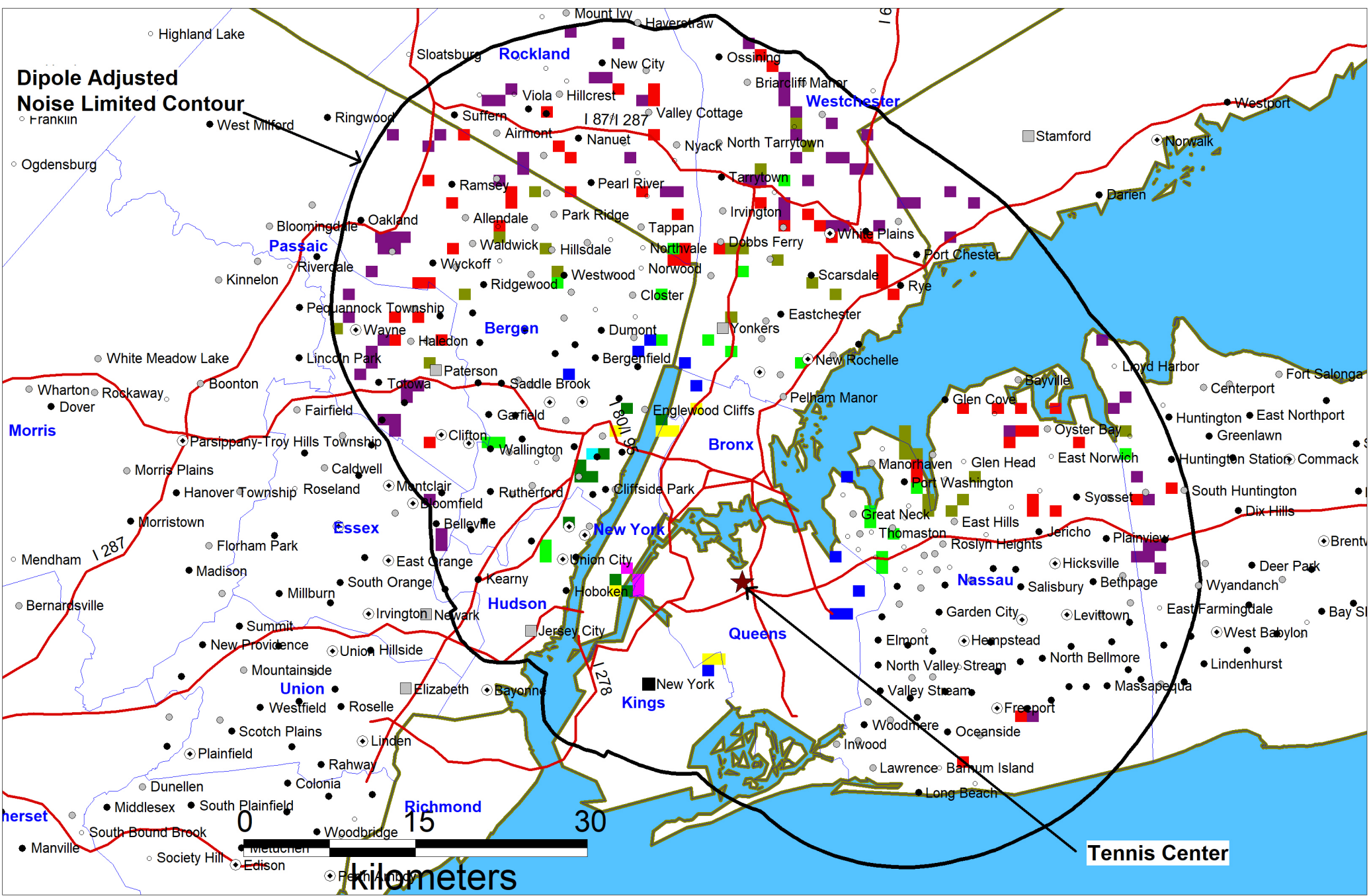
W28ES-D New York, NC CP Channel 2 Predicted Service
