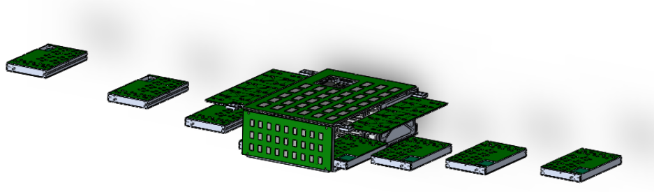
Figure 3: ANDESITE Sensor Node Deployment & Node Expanded View
