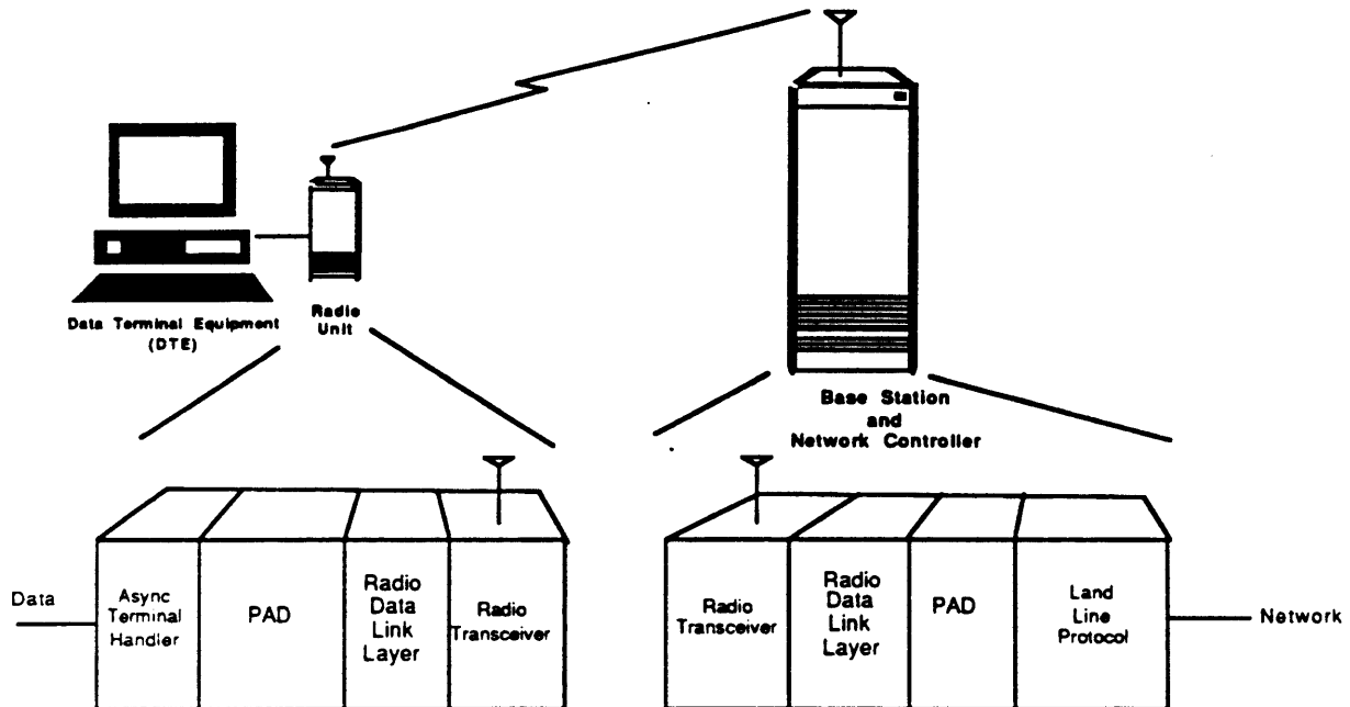
Figure 4.2 System description
