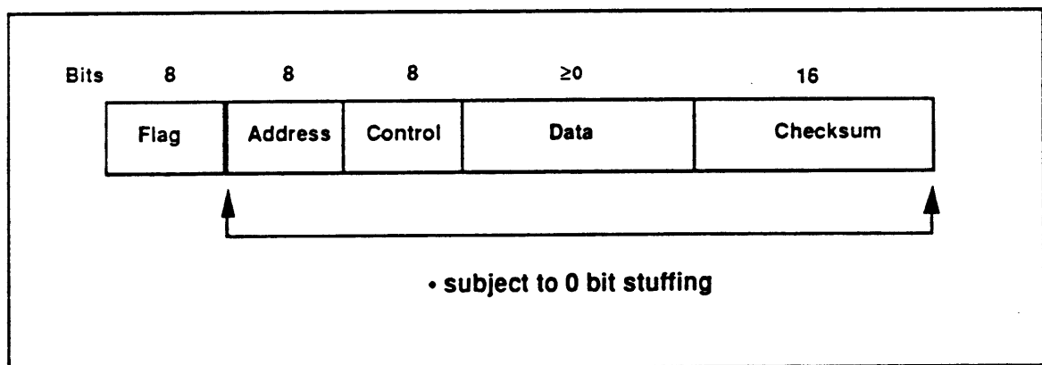
Figure 4.4 LAPB frame
