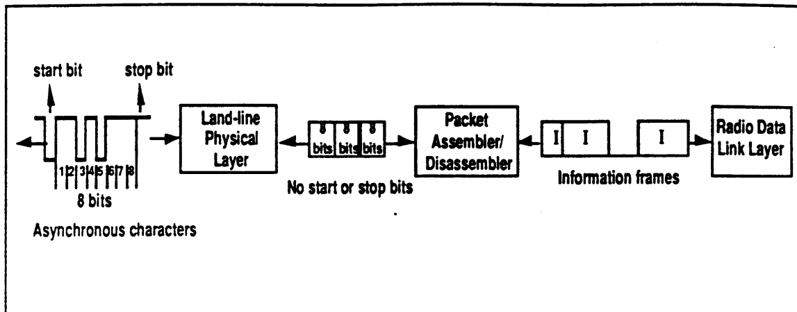
Figure 4.3 Packet Assembler/Disassembler
