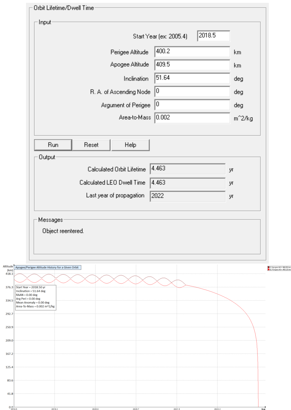
Figure 2. TEMPEST-D Orbit Lifetime/Dwell Time and Orbit Decay
