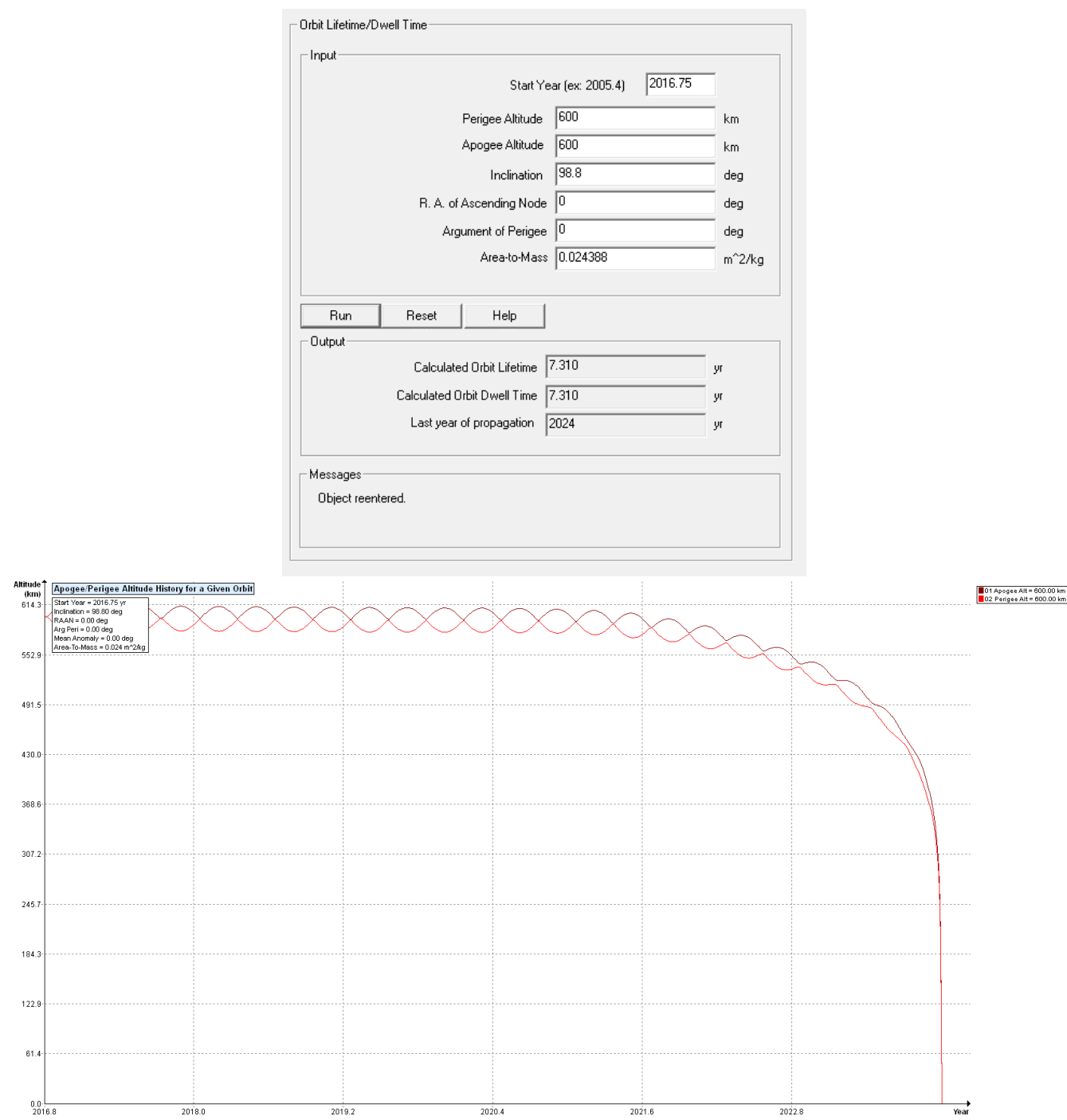
Figure 2. RAVAN Orbit Lifetime/Dwell Time and Orbit Decay
