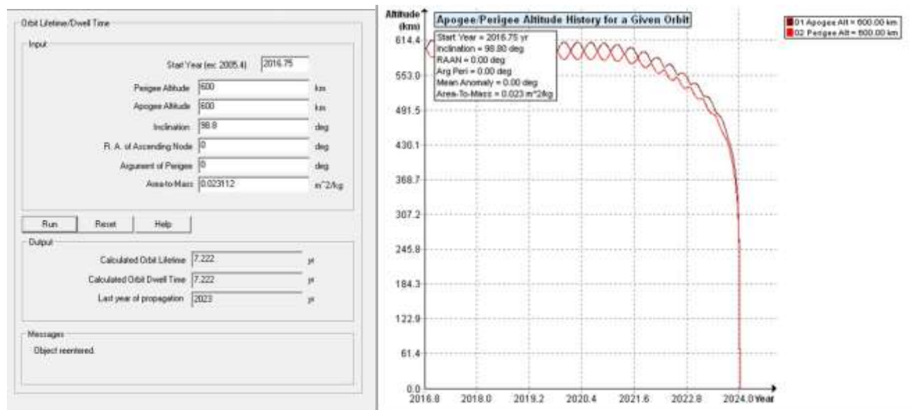
Figure 2. RAVAN Orbit Lifetime/Dwell Time and Orbit Decay
