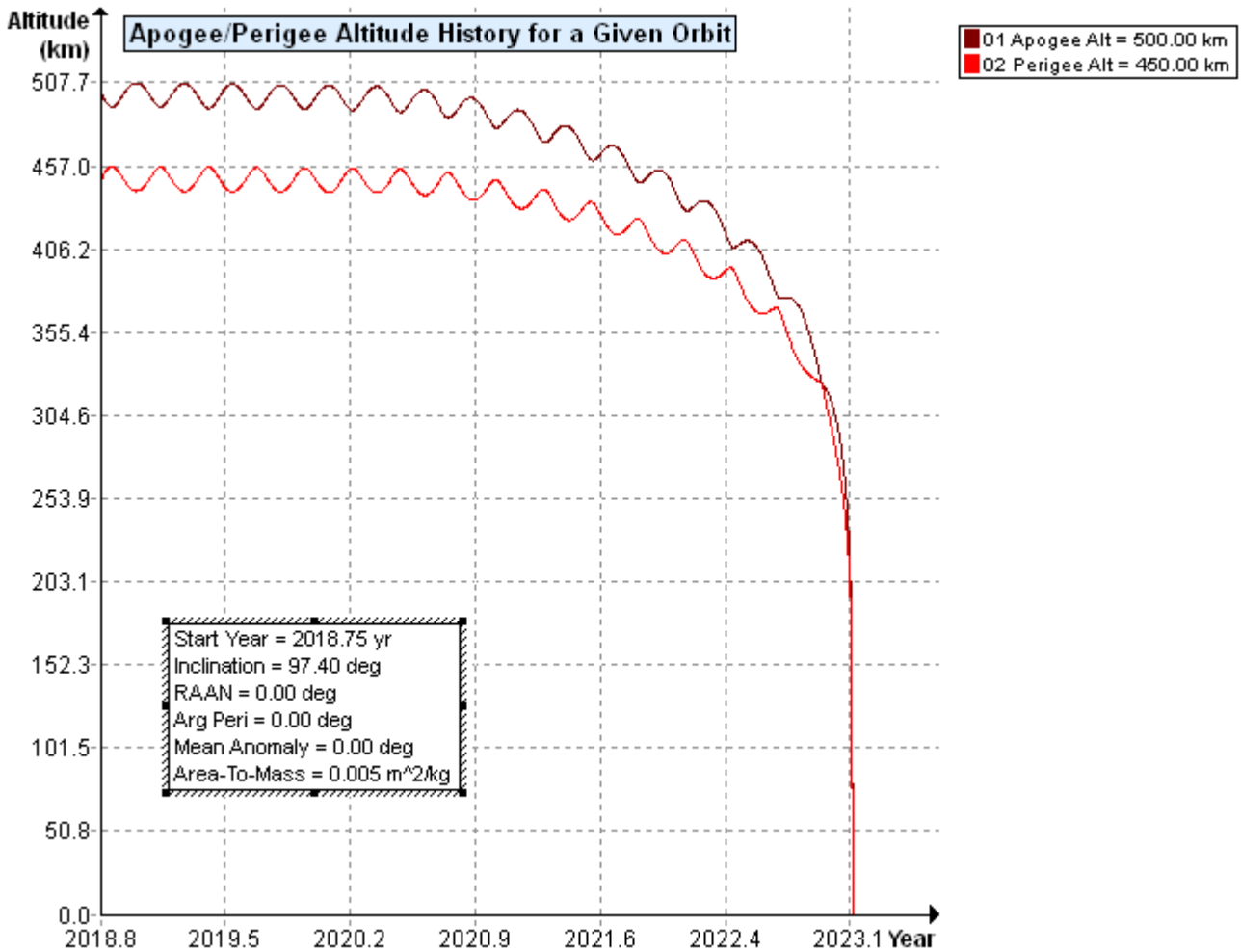
Figure 2 PATHFINDER orbit history with apogee (brown) & perigee (red)
