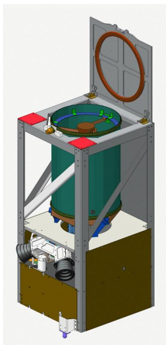
Figure 1. CAD model of the PATHFINDER spacecraft in its operational configuration.
