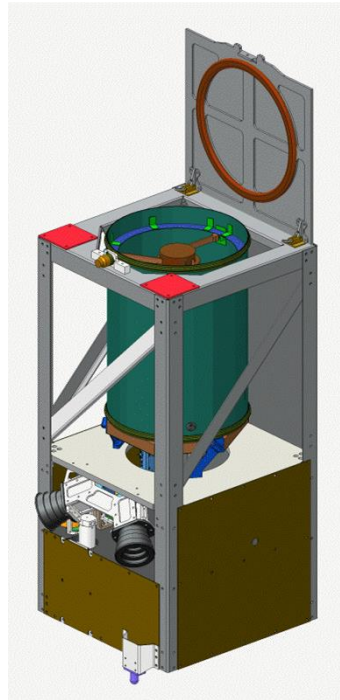
Figure 1. CAD model of the PATHFINDER spacecraft. It's launch and operational configuration are identical.
