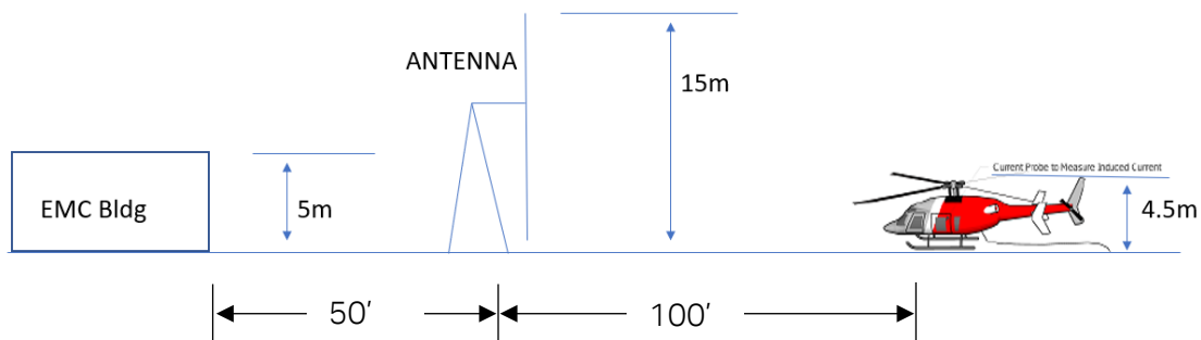
Figure 2: Large Dipole Antenna in the Vertical Configuration
