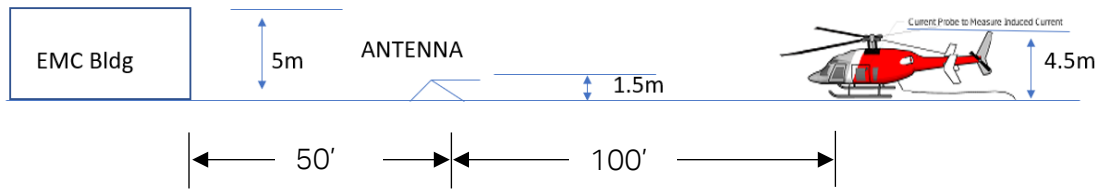
Figure 3: Large Dipole Antenna in the Horizontal Configuration
