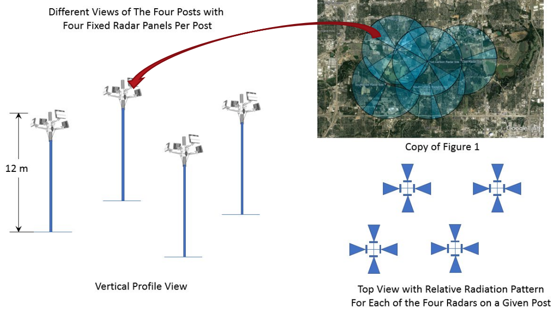
Figure 2: Additional Views Showing Radar Mast Arrangements
