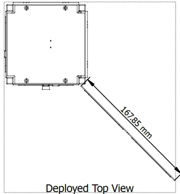
Figure 3: Audacy Zero top view drawing of deployed solar array
