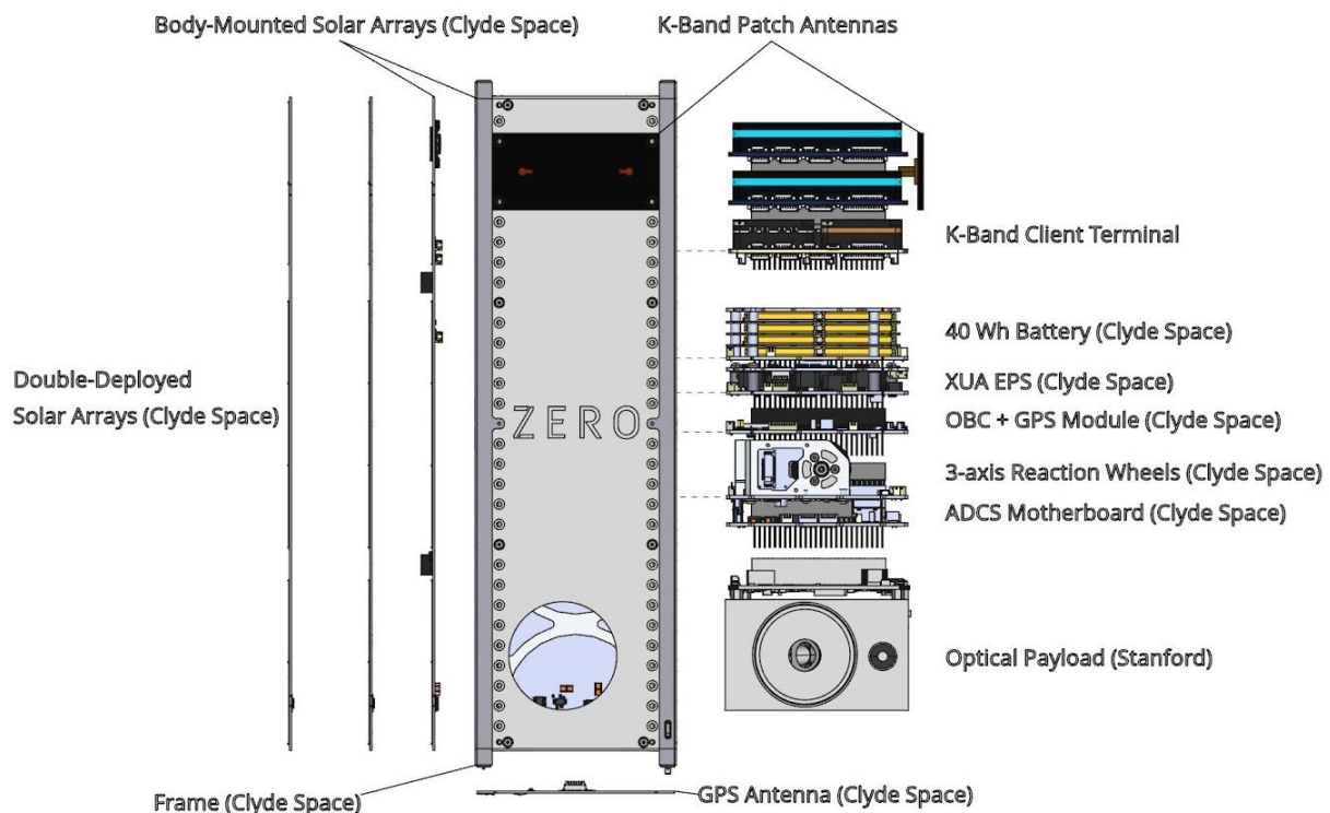
Figure 1: Audacy Zero exploded view with subsystem labels.
