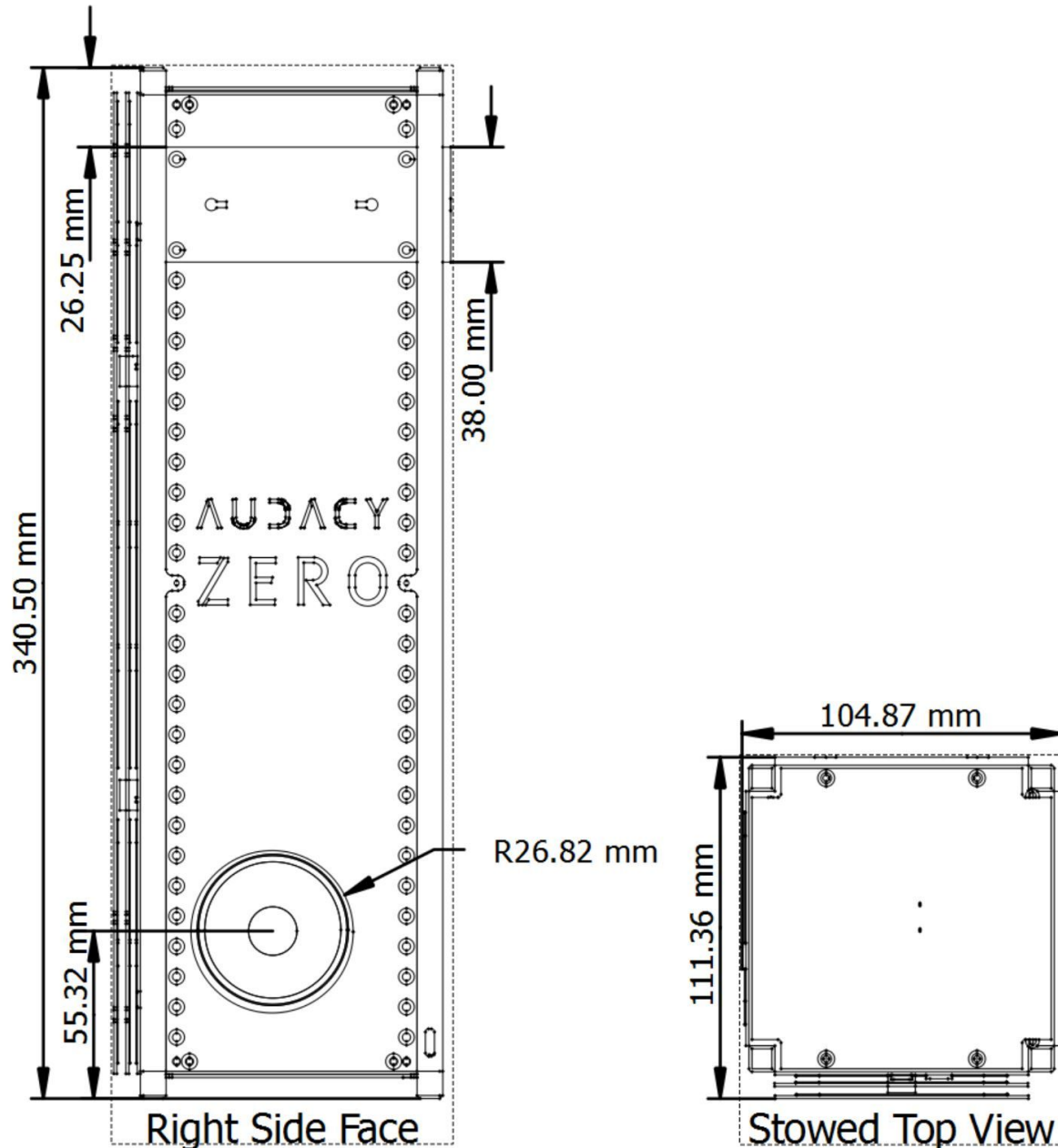
Figure 2: Audacy Zero drawings in the stowed configuration (deployable solar array)
