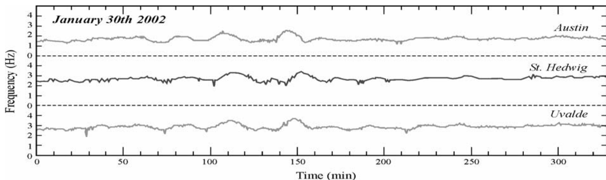
Figure 1: TIDs on three propagation paths for 4.5 MHz sounding frequency on January 30 th , 2002.
