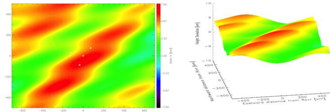
Figure 1. Reconstruction of isoionic contours perturbed by various TID components measured by the TIDDBIT TID Mapping System. Color scale represents height perturbation from -7\text{km} to +7\text{km} . Left panel: horizontal distribution centered on TIDDBIT array (white dots) and extrapolated out to several hundred kilometers. Right panel: 3-D representation of left panel. Consecutive frames can be viewed as a movie showing TIDs propagating with time.
