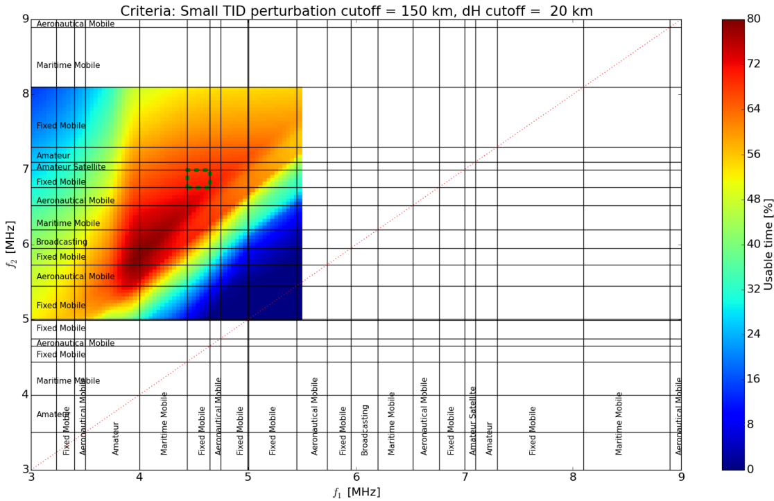
Figure 4: Optimization analysis for frequency selection. The color represents the percent of time that the two frequencies can provide robust scientific data for the duration of the experiment.
