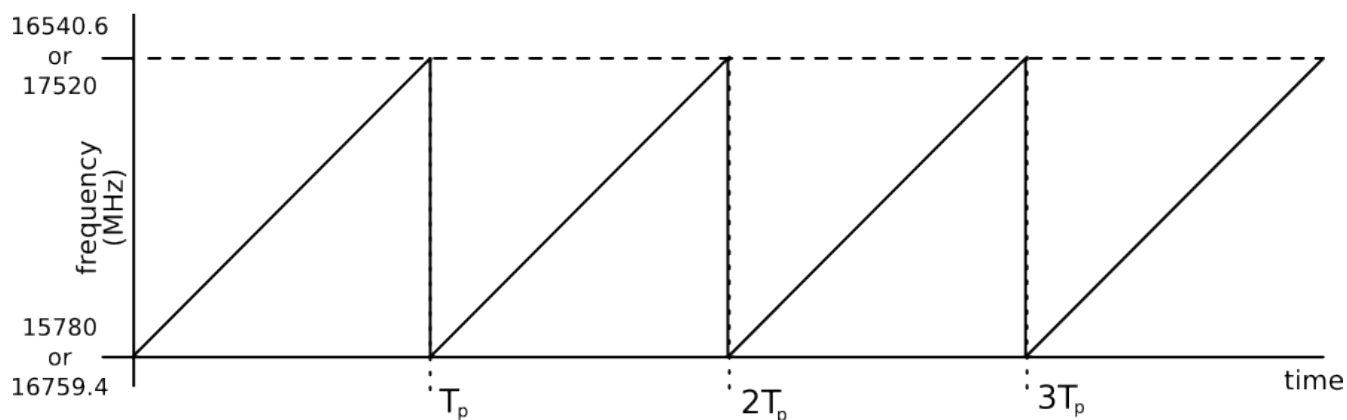
Illustration 1: Spectrogram of the SlimSAR-Ku transmitted signal.
