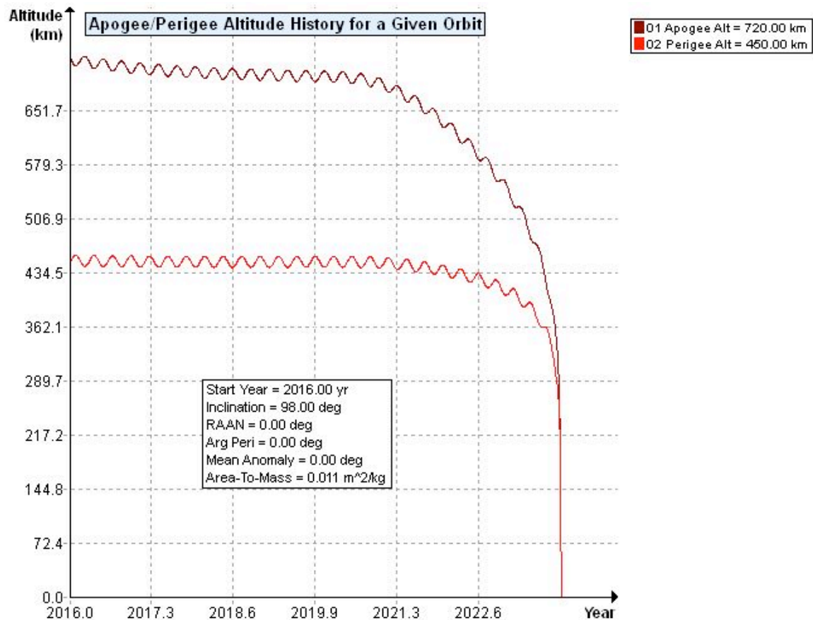
Figure 2: Corvus-BC3 Orbit History
