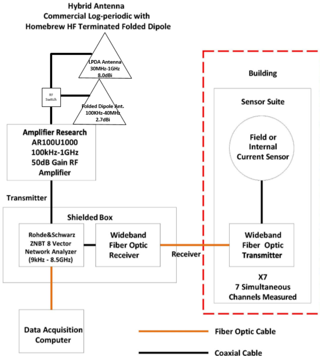
Figure 3. Functional Diagram of MIL-STD-188-125-1 or -2 Continuous Wave Immersion (CWI) Test Setup (Network Analyzer Measures S21, S31, S41, etc. Simultaneously)
