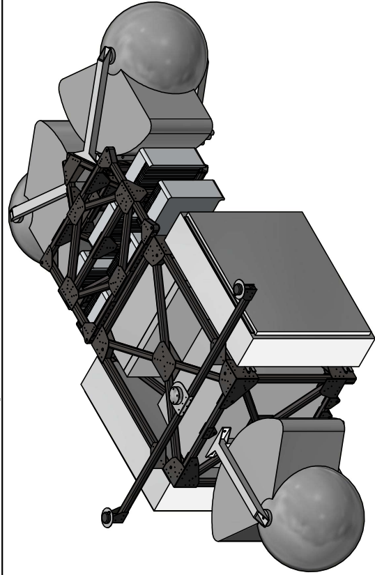
ALTAEROS AVIONICS AND PAYLOAD FRAMES WITH AVIONICS AND PAYLOAD COMPONENTS
