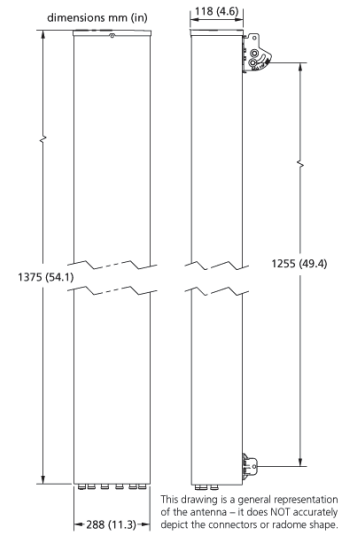
Antenna Drawing
