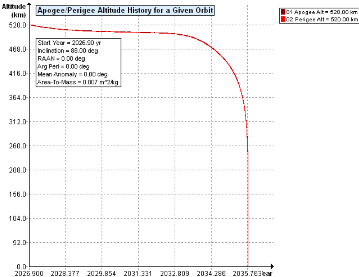
Figure 6.1. Titan De-orbit Altitude Profile from Operational Altitude
