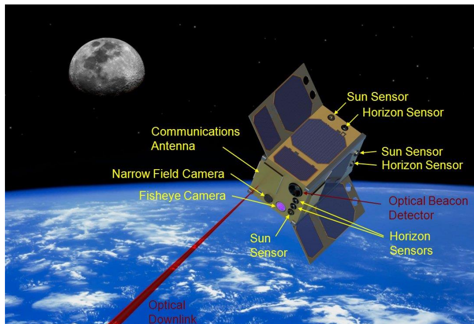
Figure 1. The AeroCube-7 spacecraft with optical downlink beam, assorted sensors, and antenna.
