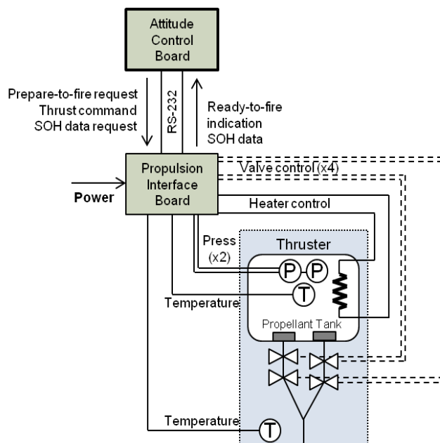
Figure 2. Schematic of the AeroCube-7 warm-gas propulsion system.
