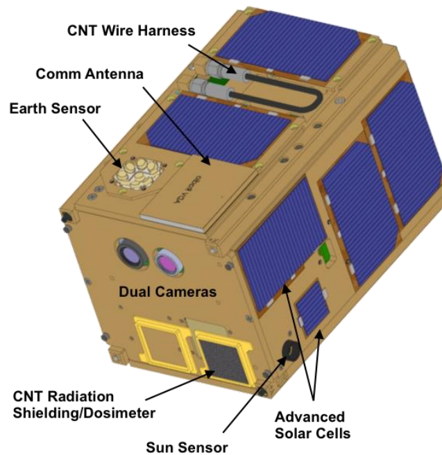
Figure 1. The AeroCube-8 spacecraft with radiation shield, assorted sensors, solar cells, and antenna.
