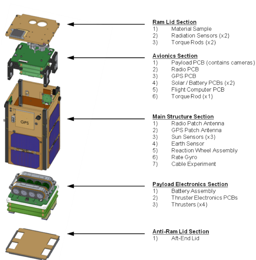
Figure 2. Exploded isometric view of AeroCube-8.
