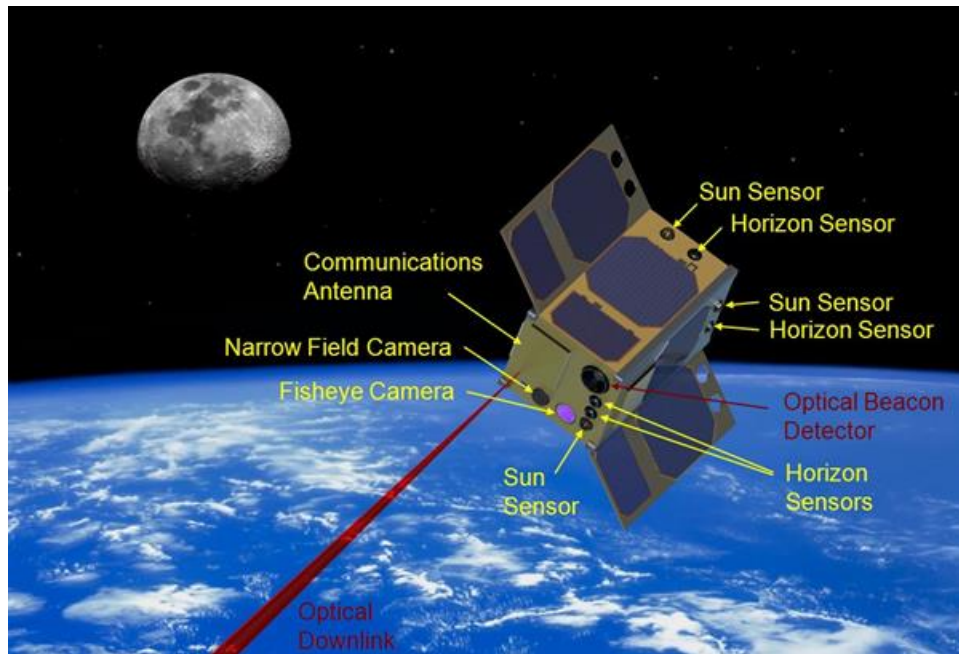
Figure 1. The AeroCube-7 spacecraft.
