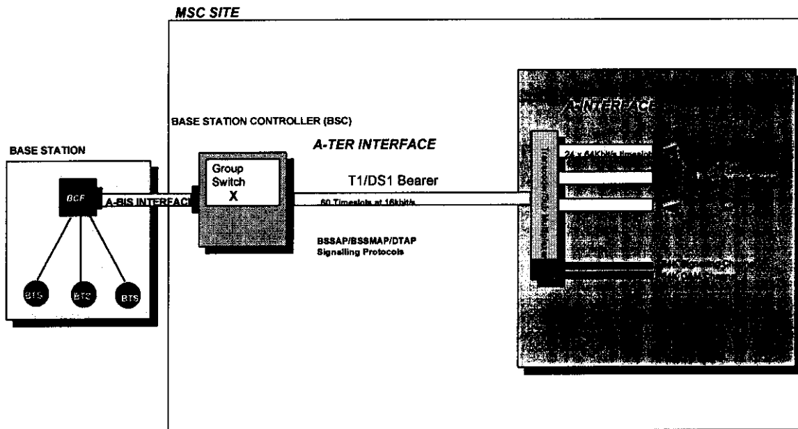
Diagram 1 Base Station Subsystem (BSS) Architecture
