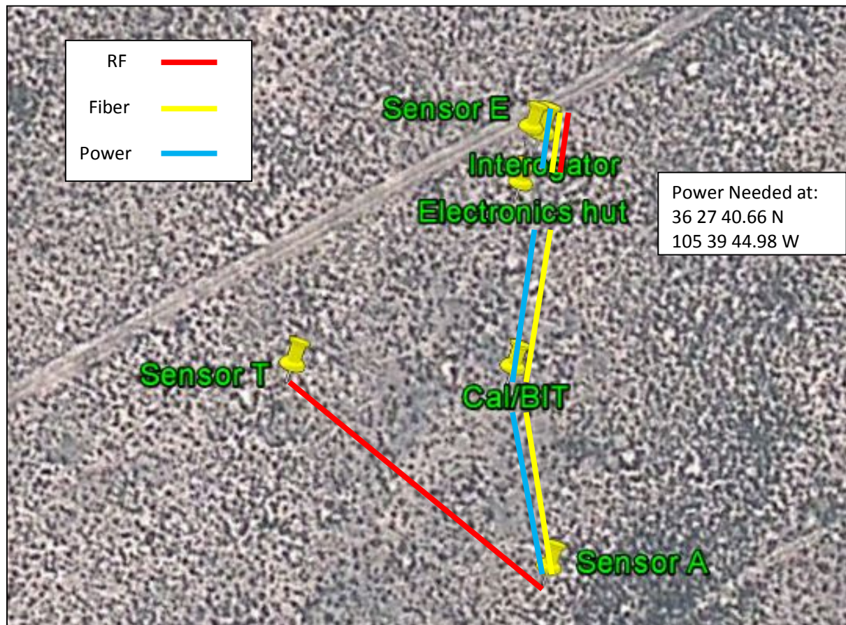
Figure 1 – cable schematic for TPMS at TAOS Regional
