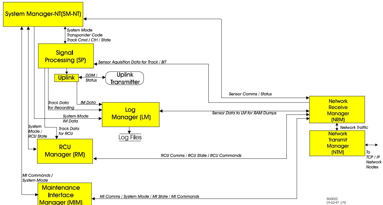
Figure 28 Base CPU2 Architecture
