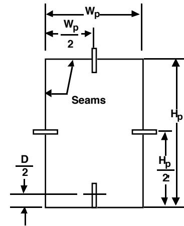
d) Panel seam measurements
