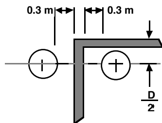
e) Partially accessible corner seam measurements
