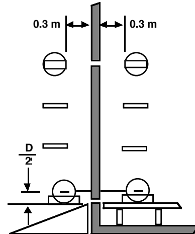
b) Door measurements
