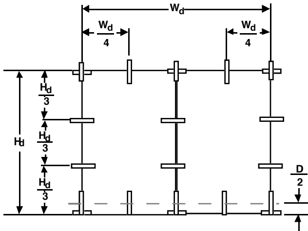
c) Double-panel entry door measurements
