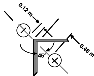
f) Fully accessible corner seam measurements
