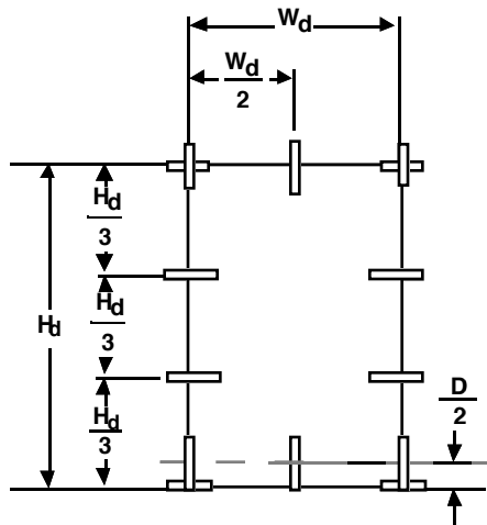
a) Single-panel entry door measurements
