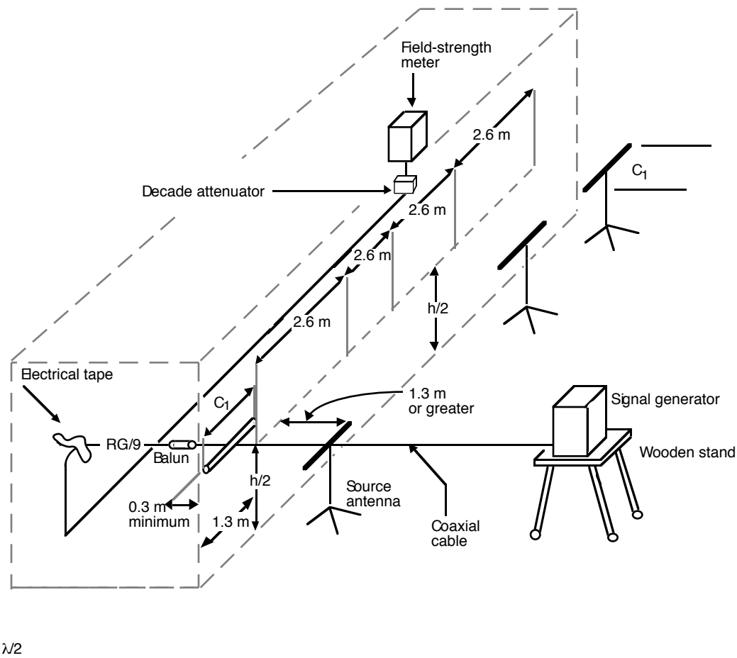
Figure 7—Measurement setup for frequencies \leq 1000 MHz
