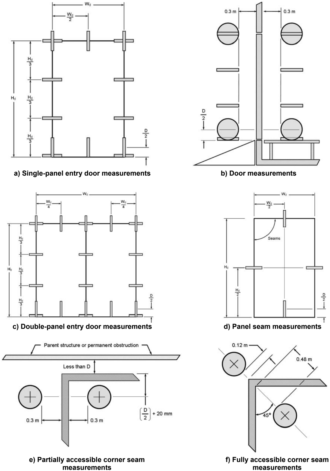
Figure 2—Standard loop positions for low-frequency tests
