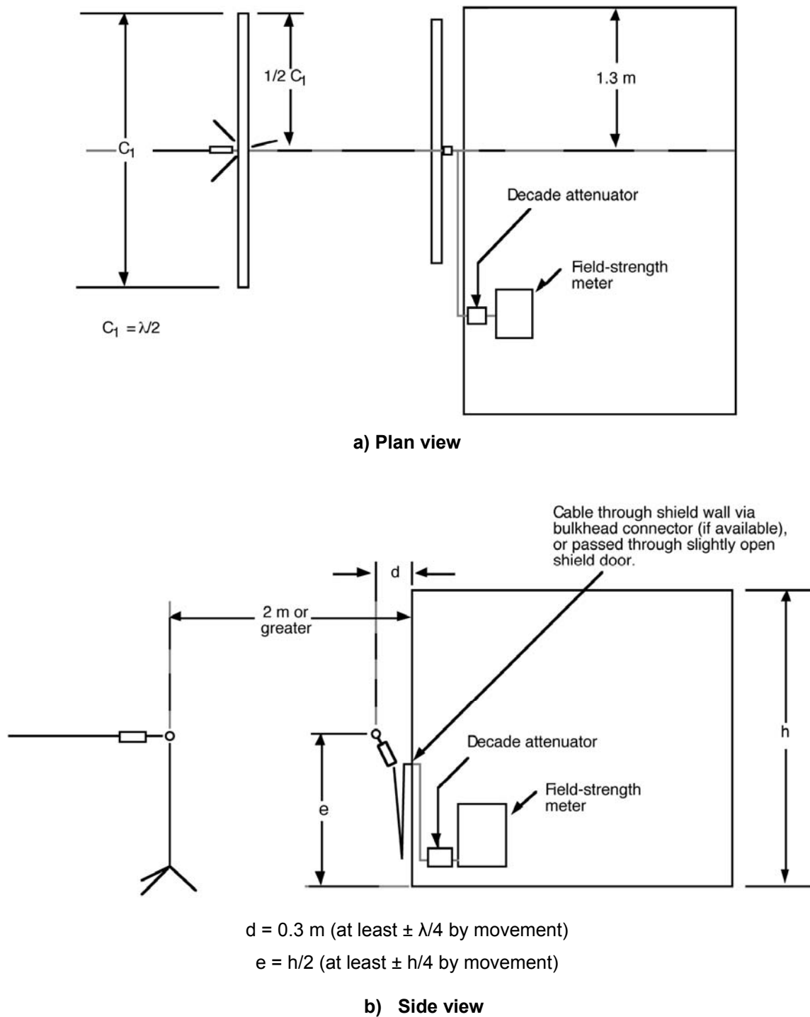
Figure 6—Reference setup for frequencies \leq 1000 MHz
