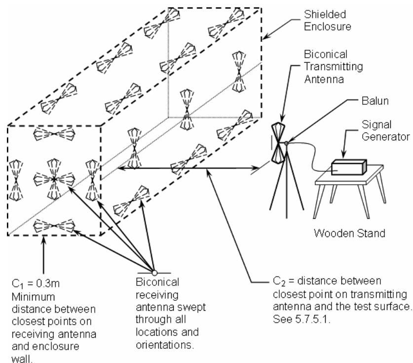
b) Measurement setup (vertical transmitting antenna orientation), 20 MHz–100 MHz
