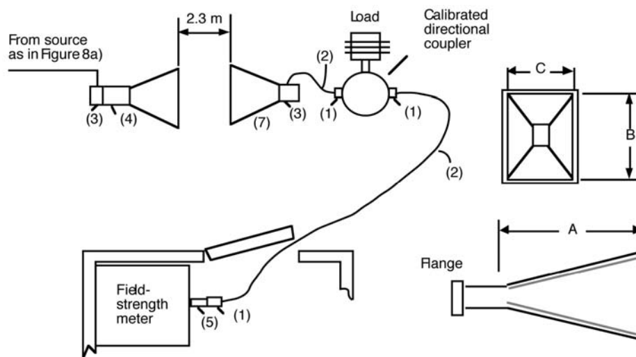
b) Enclosure free-field simulation
