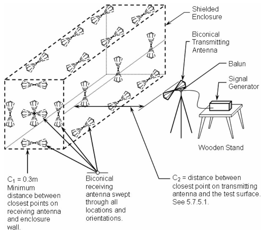
a) Measurement setup (horizontal transmitting antenna orientation), 20 MHz–100 MHz
