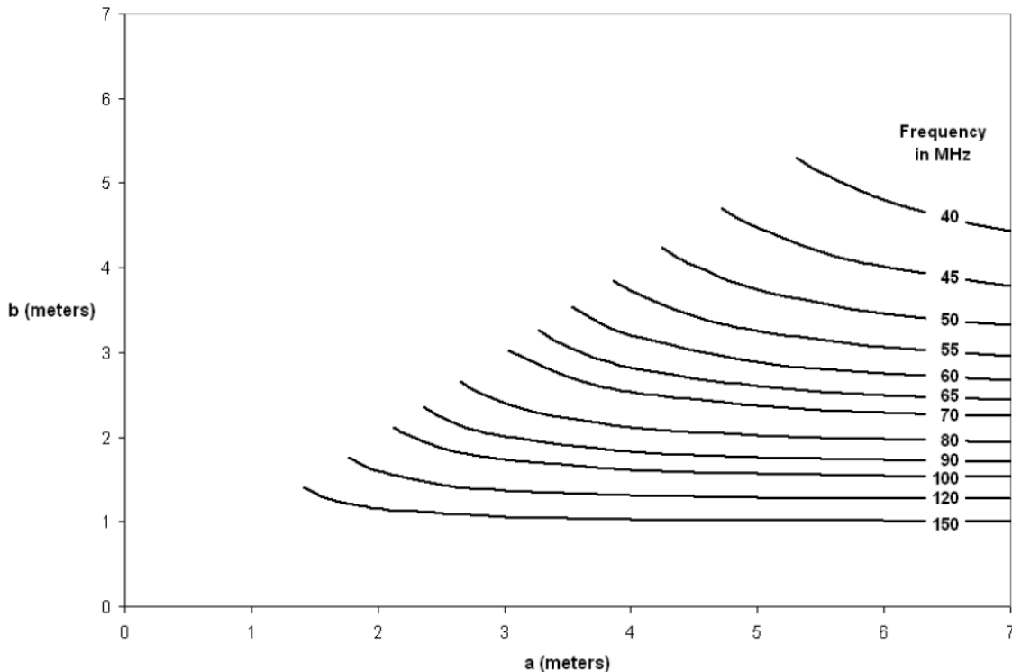
Figure 5—Lowest natural resonant frequency chart
