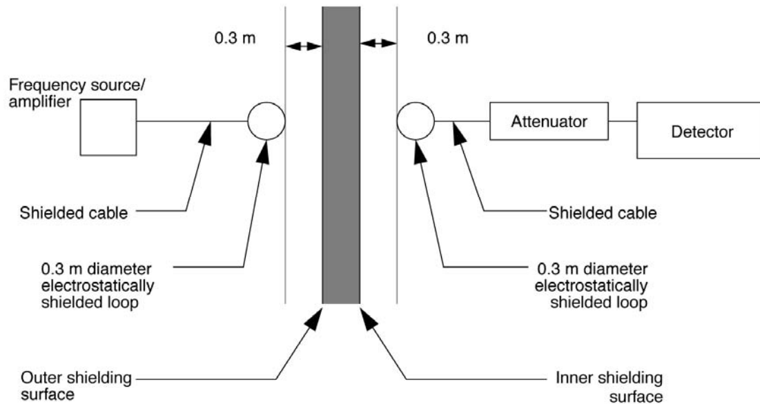
Figure 1—Schematic diagram of the test configuration for magnetic tests showing dimensions of transmit and receive antennas (coplanar antenna orientations)
