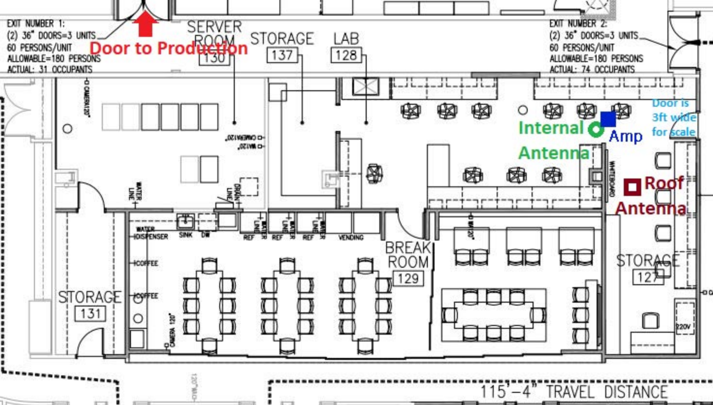
50 ft. LMR-400 connecting roof antenna and amplifier/internal antenna
