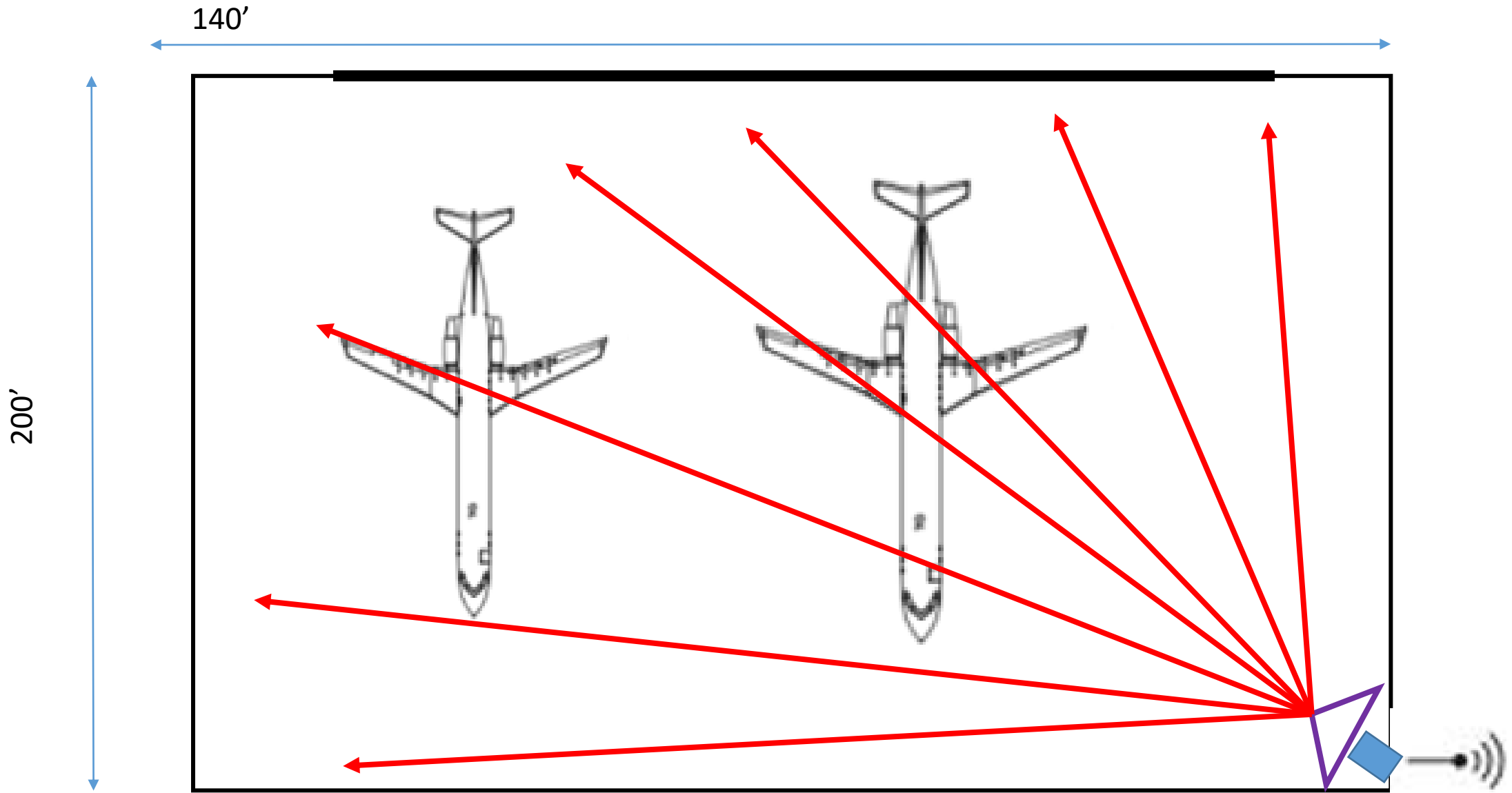
External antenna connected to amplifier via 100 ft. of LMR-240
