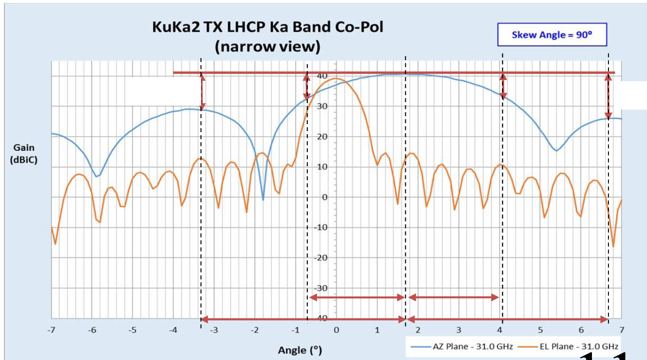
Figure 4: Measured LHCP Transmit Terminal Antenna narrow pattern cuts (+/- 7.0 deg) for worst case Skew angle 90 deg. These patterns are measured with radome.
