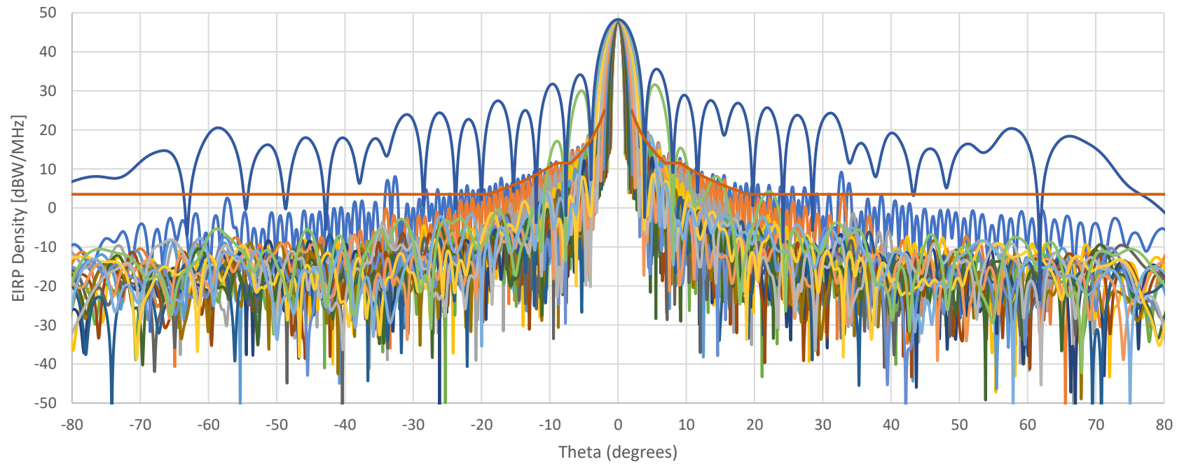
Viasat Global Aero Terminal (GAT) 5530 EIRP Density Plot at 29.25 GHz
