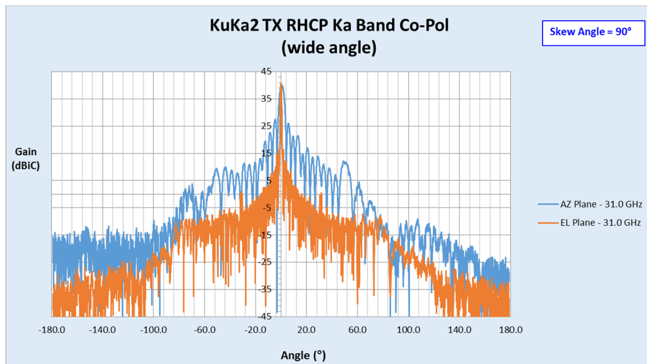
Figure 1: Measured RHCP Transmit Terminal Antenna wide pattern cuts for worst case Skew angle 90°. These patterns are measured with radome.
