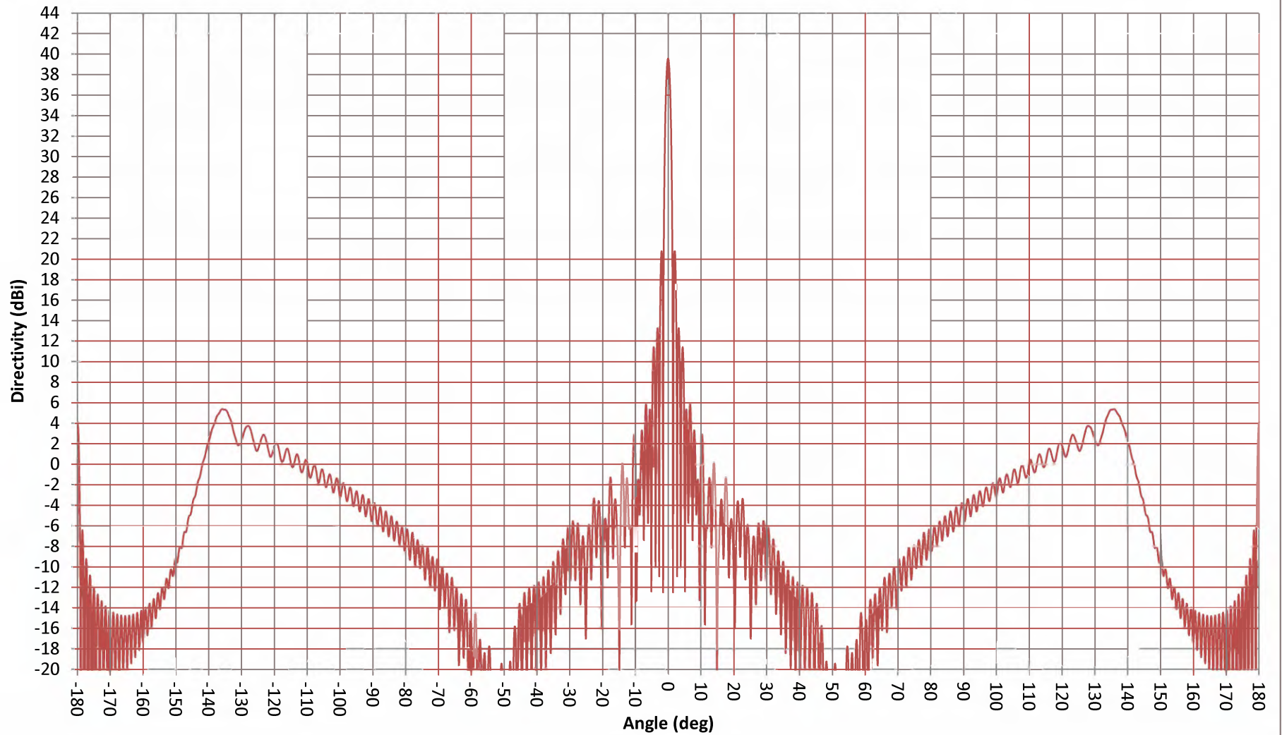
ViaSat Antenna Range 4 ft Diam Transmit Antenna Calculated Secondary Pattern 12 GHz Model 23-4 Refl Model 28-12 Feed Vert Pol
