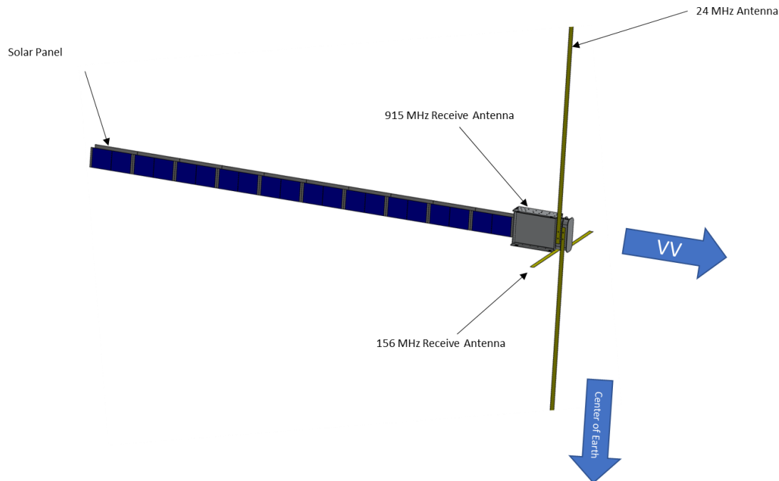
Figure 1 VariSat-1 Overview
