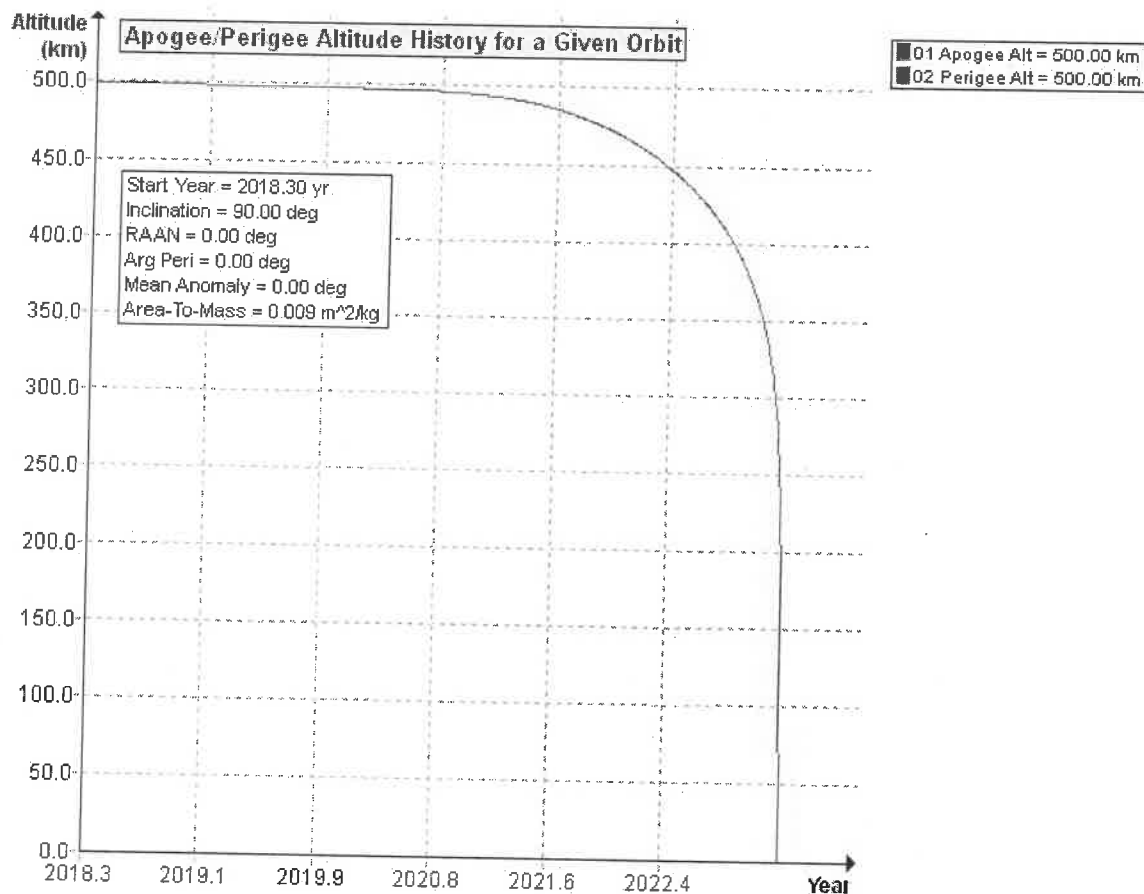
Figure 3: TechEdSat-7 Orbit History for Case 2: Failed Deployment
