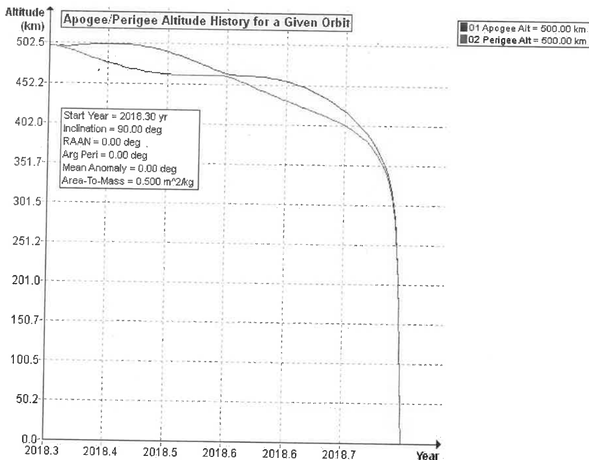
Figure 2: TechEdSat-7 Orbit History for Case 1: Nominal Deployment
