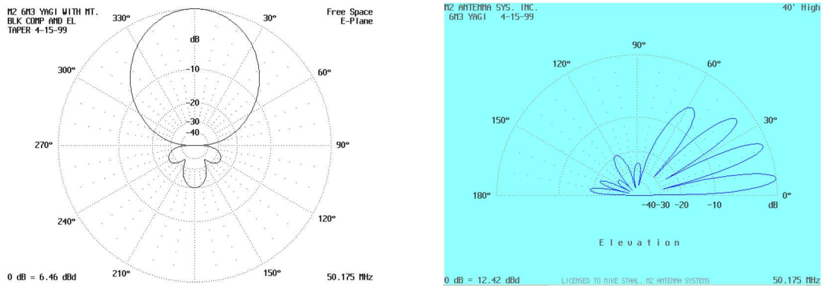
Figure 7: The M2 Inc. [36] (6.4 dBd gain) antenna is the transmitting antenna used in this experiment.
