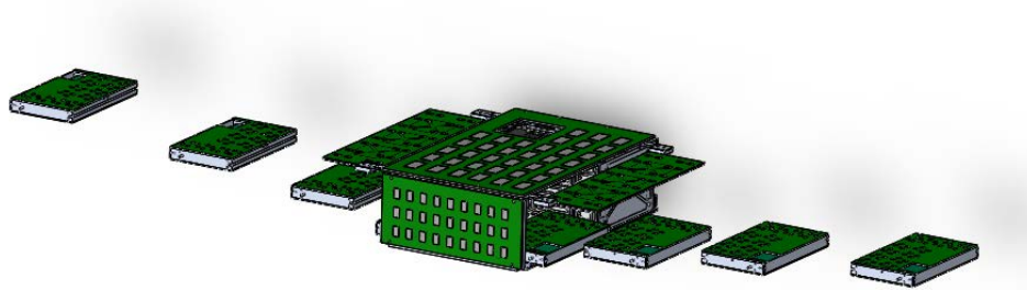
Figure 3: ANDESITE Sensor Node Deployment & Node Expanded View
