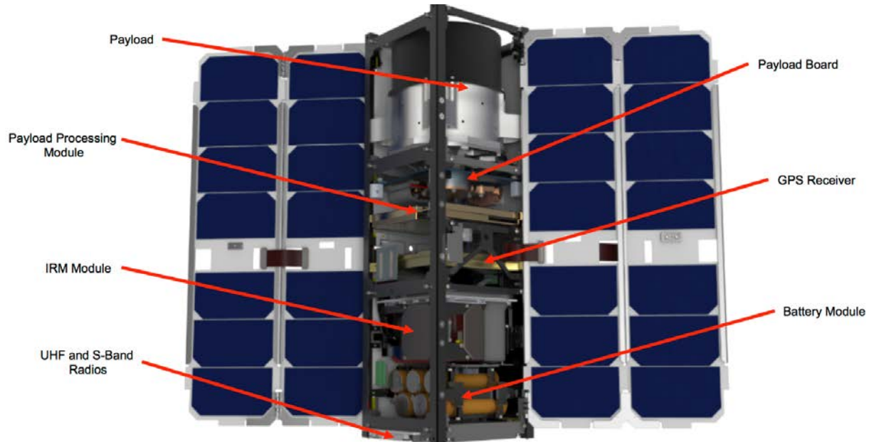
Figure 17: CubeSat X Expanded View
