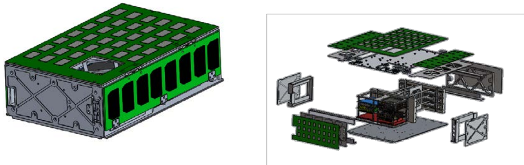
Figure 2: ANDESITE System and Expanded View
