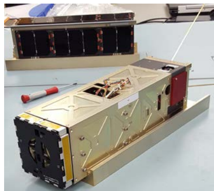
Figure 20: SHFT 3U Cube-sat Stowed configuration
