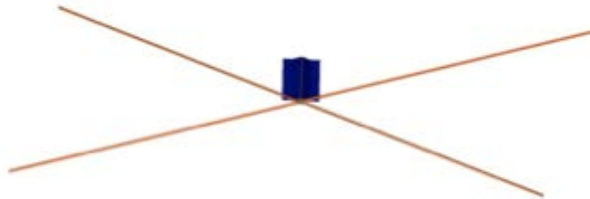
Figure 19: SHFT 3U Cube-sat Deployed view with 3 meter HF antennas
