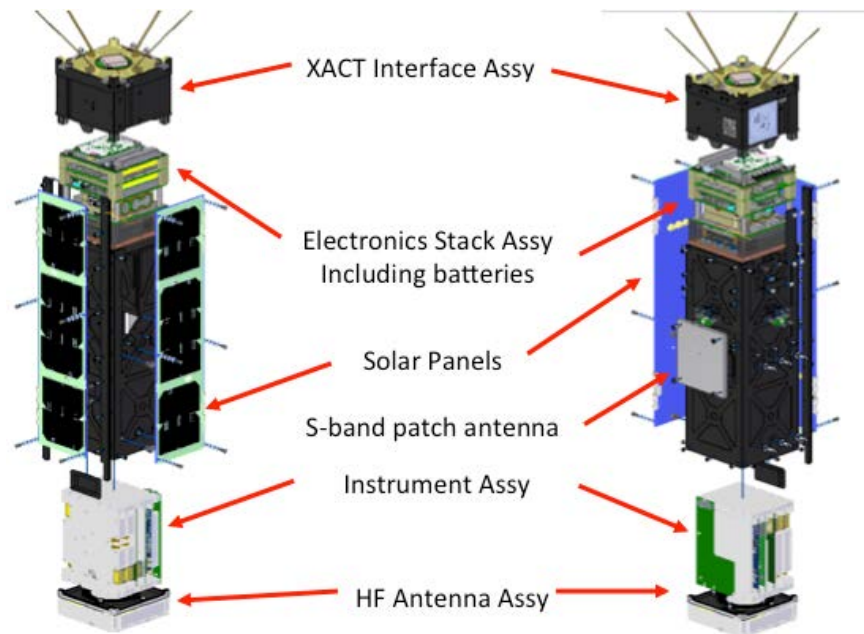
Figure 18: SHFT 3U Cube-sat Expanded View
