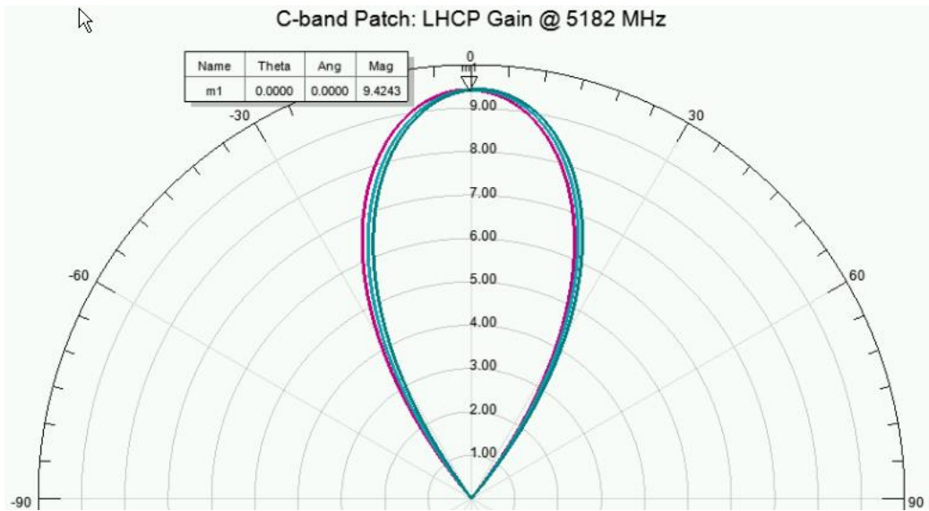
C-Band Patch Antenna LHCP Gain (Green: \theta = 0^\circ , Blue: \theta = 45^\circ , Purple: \theta = 90^\circ )
