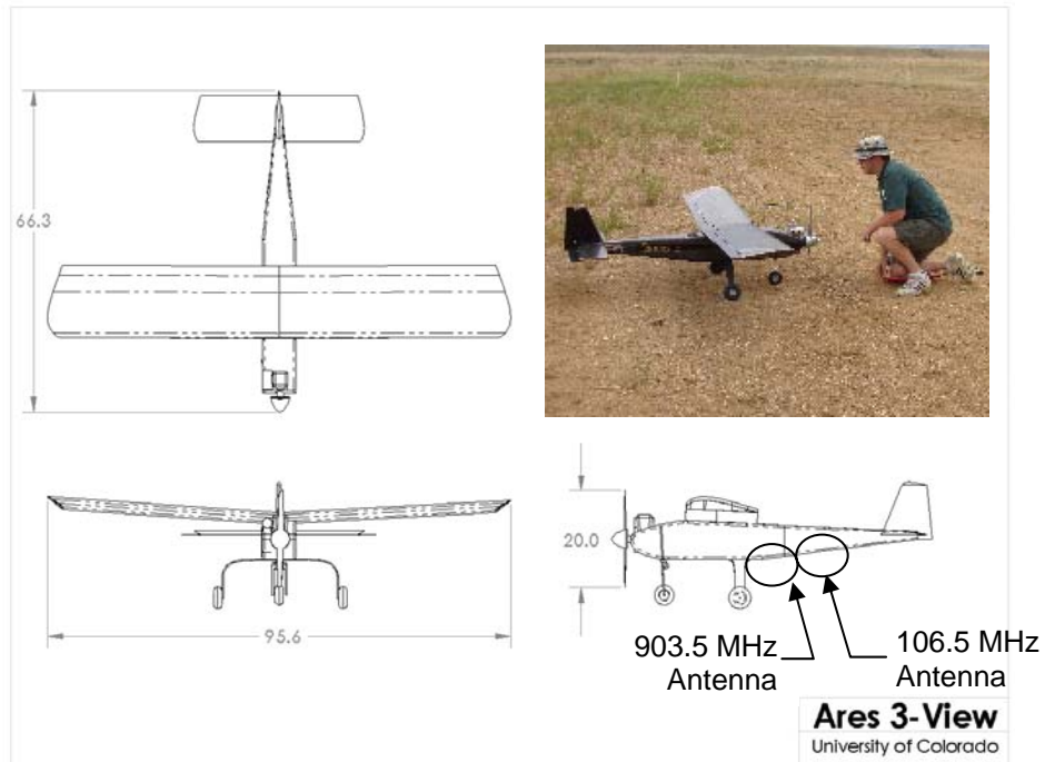
Figure 1: Ares UA. Dimensions in inches.
