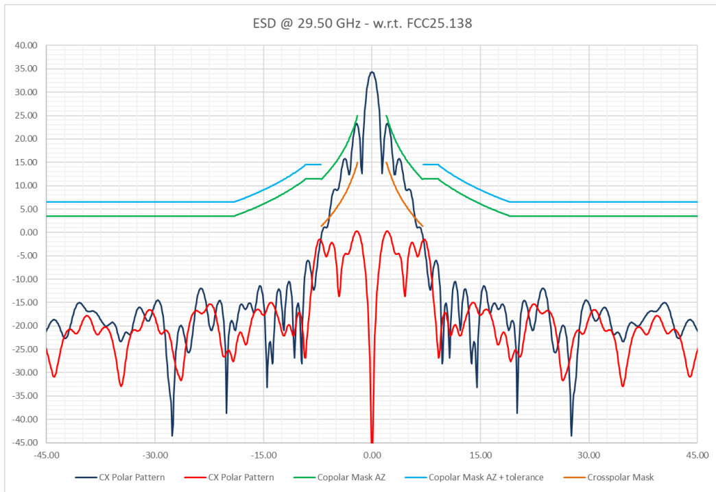
Figure 3-5 – ESD Pattern for CO and CX Patterns w.r.t. FCC 25.138 Applicable Standard @ 29.50 GHz
