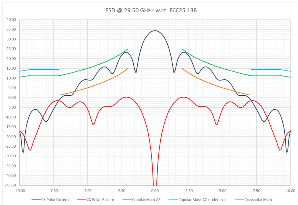
Figure 3-6 – ESD Pattern for CO and CX Patterns w.r.t. FCC 25.138 Applicable Standard @ 29.50 GHz
