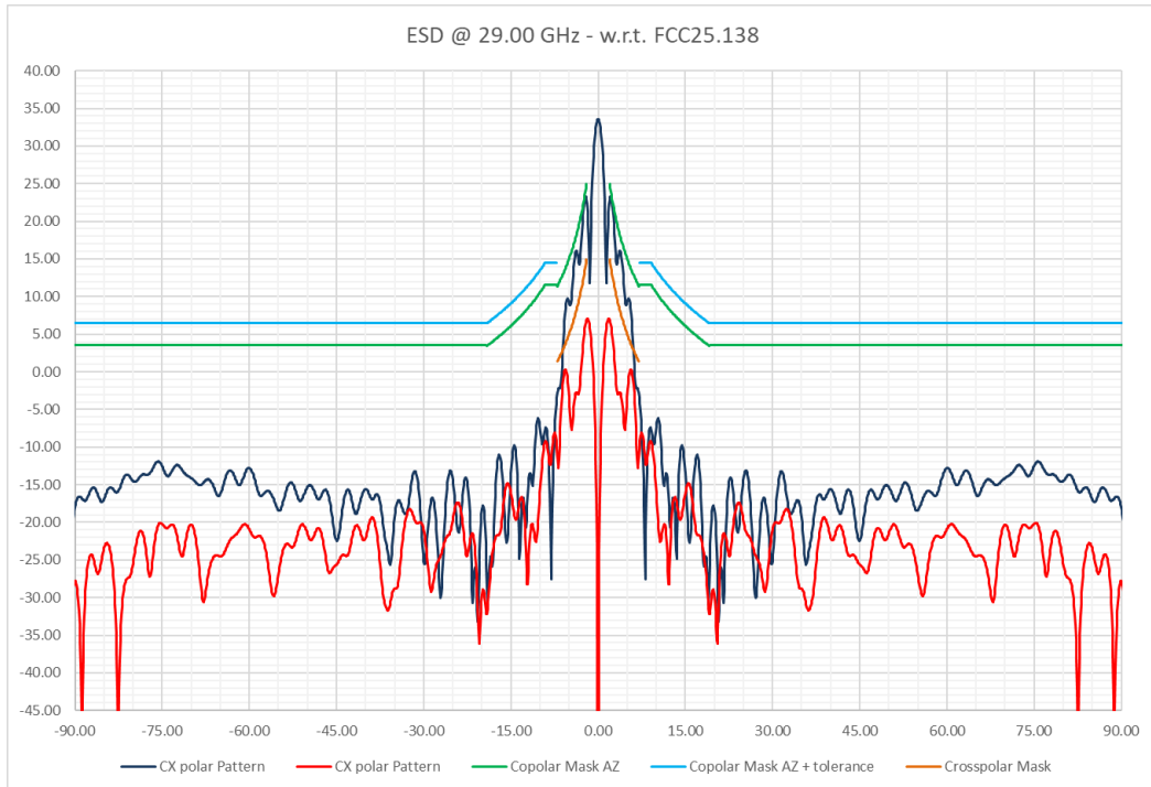
Figure 3-1 – ESD Pattern for CO and CX Patterns w.r.t. FCC 25.138 Applicable Standard @ 29.00 GHz
