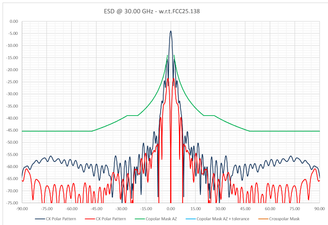
Figure 3-9 – ESD Pattern for CO and CX Patterns w.r.t. FCC 25.138 Applicable Standard @ 30.00 GHz
