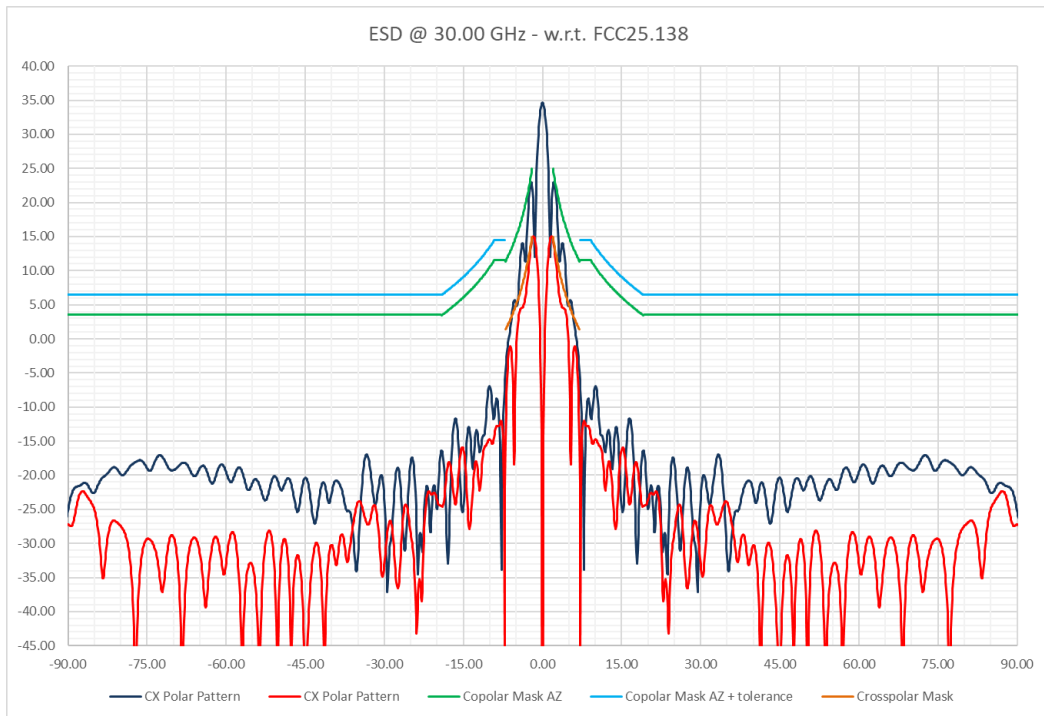
Figure 3-7 – ESD Pattern for CO and CX Patterns w.r.t. FCC 25.138 Applicable Standard @ 30.00 GHz
