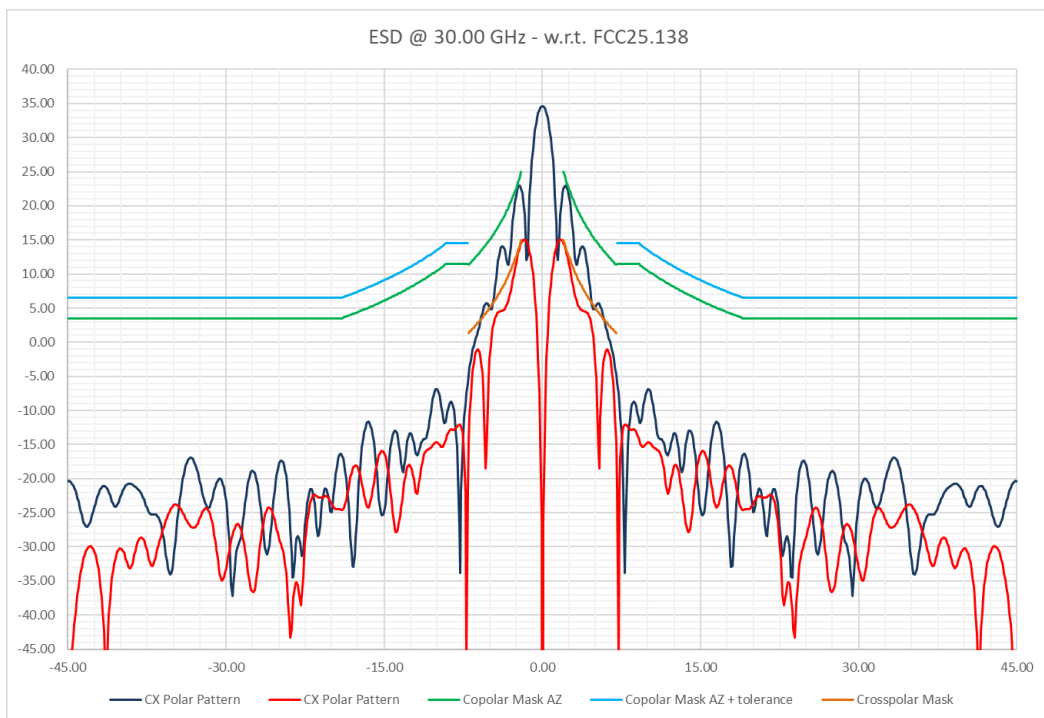
Figure 3-8 – ESD Pattern for CO and CX Patterns w.r.t. FCC 25.138 Applicable Standard @ 30.00 GHz
