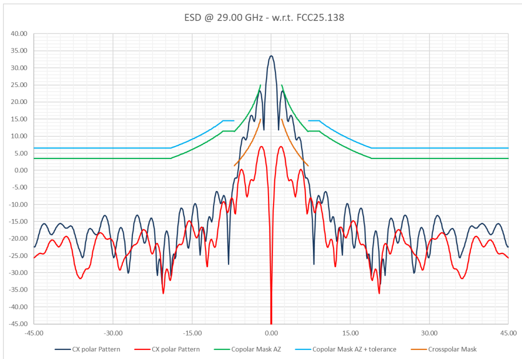
Figure 3-2 – ESD Pattern for CO and CX Patterns w.r.t. FCC 25.138 Applicable Standard @ 29.00 GHz
