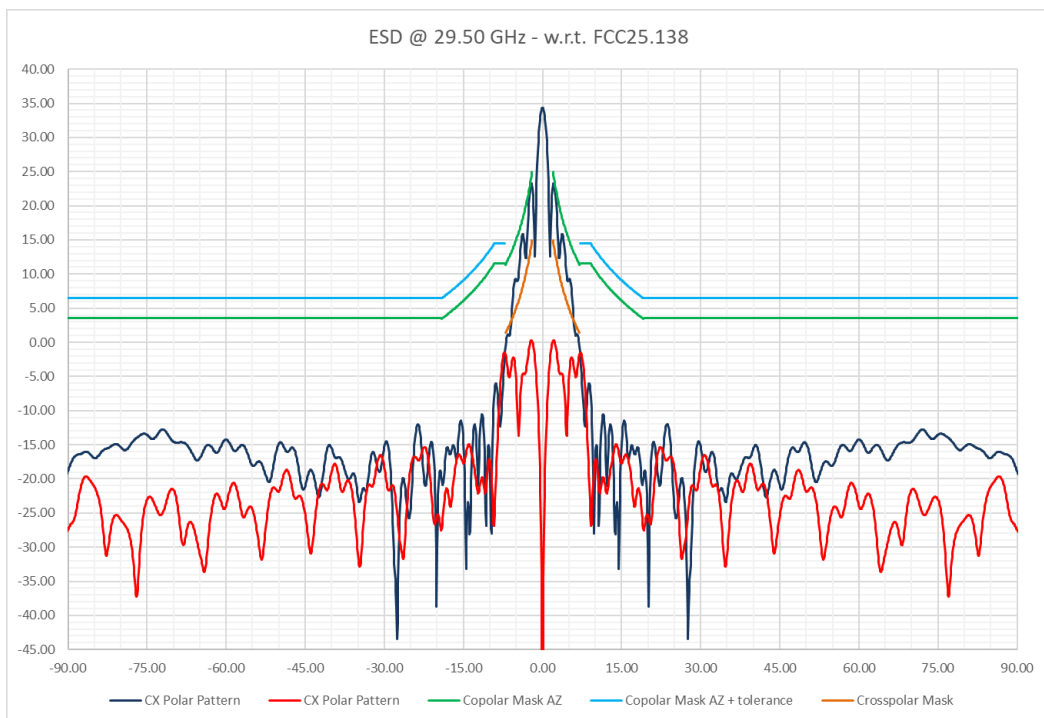
Figure 3-4 – ESD Pattern for CO and CX Patterns w.r.t. FCC 25.138 Applicable Standard @ 29.50 GHz
