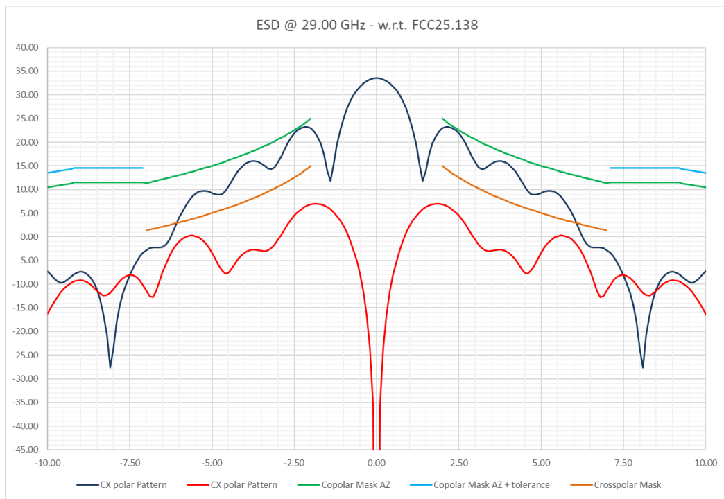
Figure 3-3 – ESD Pattern for CO and CX Patterns w.r.t. FCC 25.138 Applicable Standard @ 29.00 GHz
