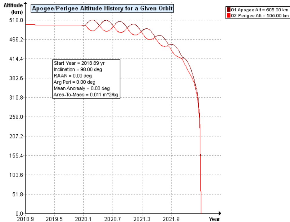
Figure 2: TYVAK-0087 Deorbit Lifetime
