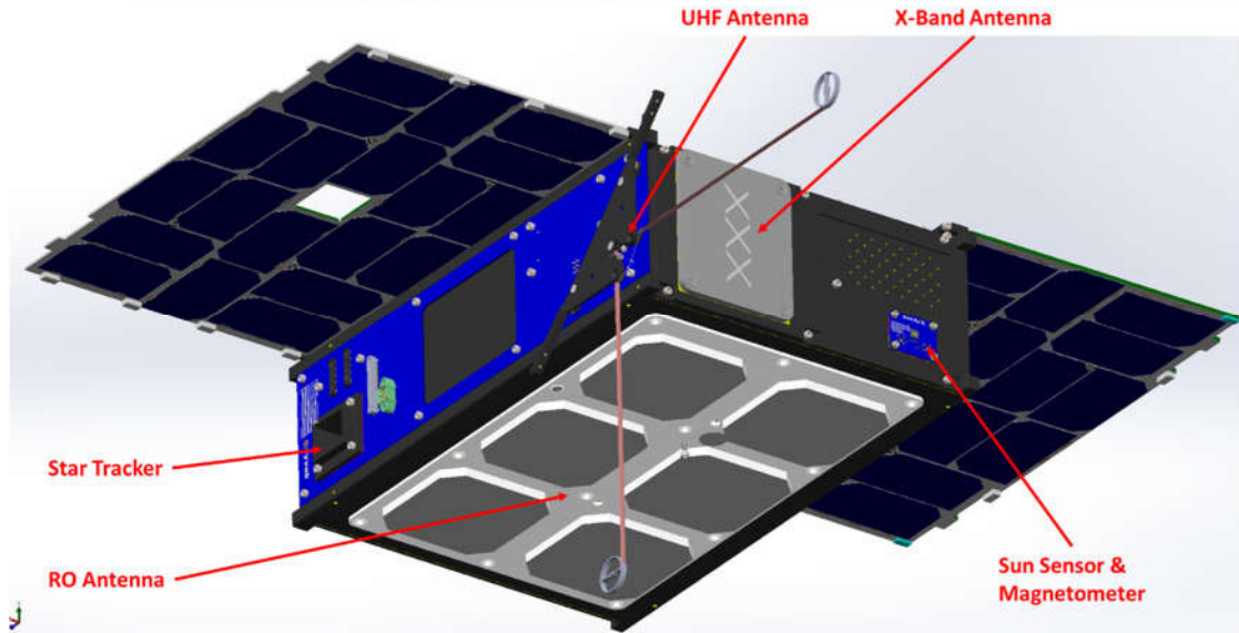
Figure 2-1: Spacecraft Vehicle Layout
