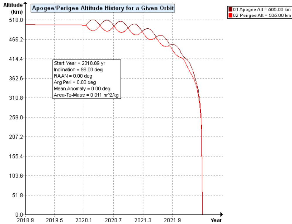
Figure 6-3: TYVAK-0087 Deorbit Lifetime
