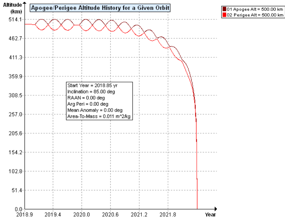
Figure 6-2: TYVAK-0086 Deorbit Lifetime
