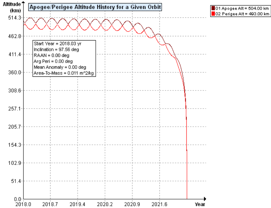
Figure 6-1: TYVAK-0085 Deorbit Lifetime
