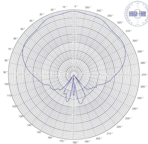
Figure 4: X-band Antenna Gain Plot
