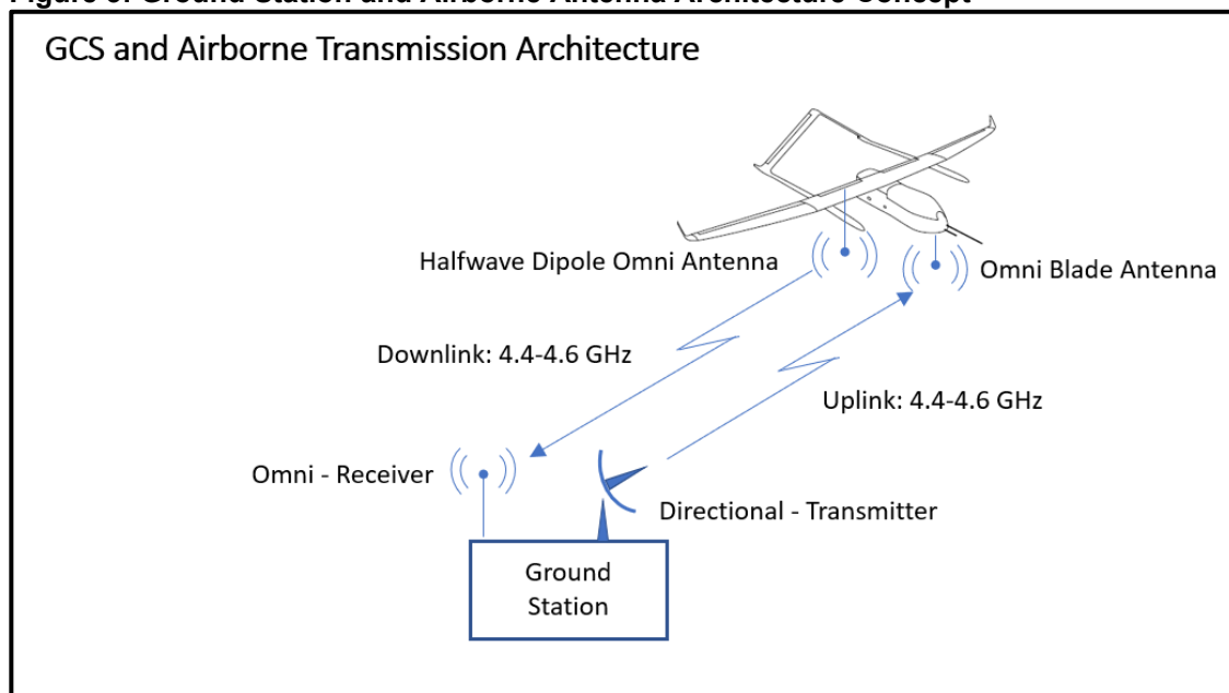
Figure 4 illustrates the airborne and ground station configuration.
