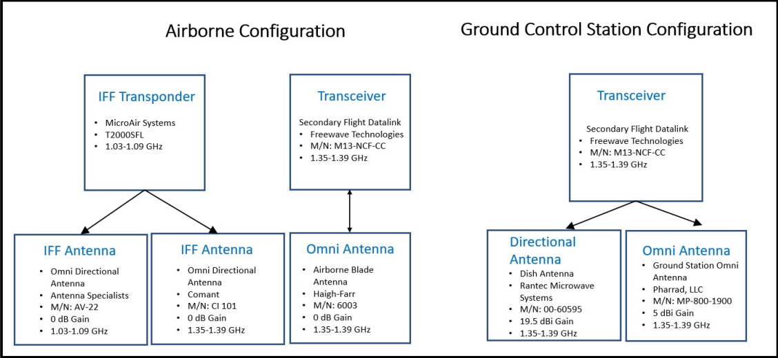
Figure 4: Airborne and Ground Station Configuration
