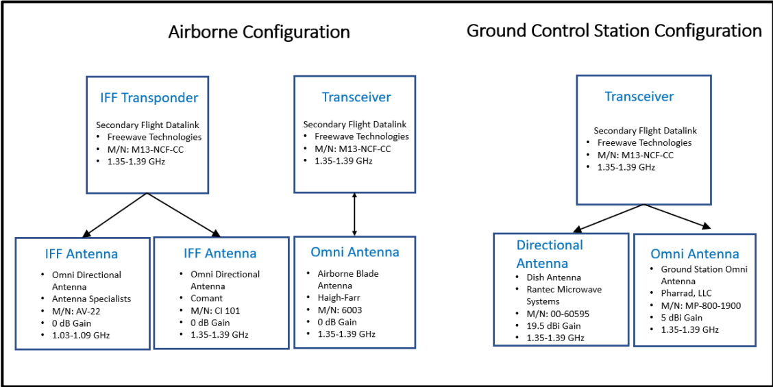
Figure 4: Airborne and Ground Station Configuration
